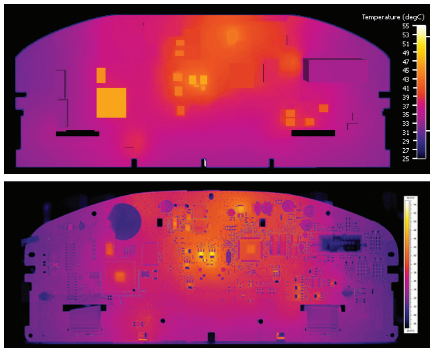
Figure 4: Comparison of CFD result during design with actual PCB measured with an IR camera.
