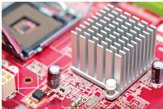
Figure 2: Heatsink extending beyond package body with retaining pins.
