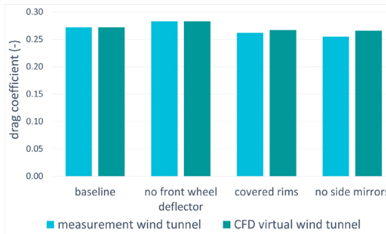
Validated digital wind tunnel results for production car aerodynamics (credit: Emil Ljungskog, doctoral thesis, "Evaluation and modeling of the flow in a slotted wall wind tunnel", 2019).
