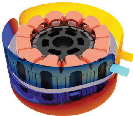
E-machine cooling simulation.
