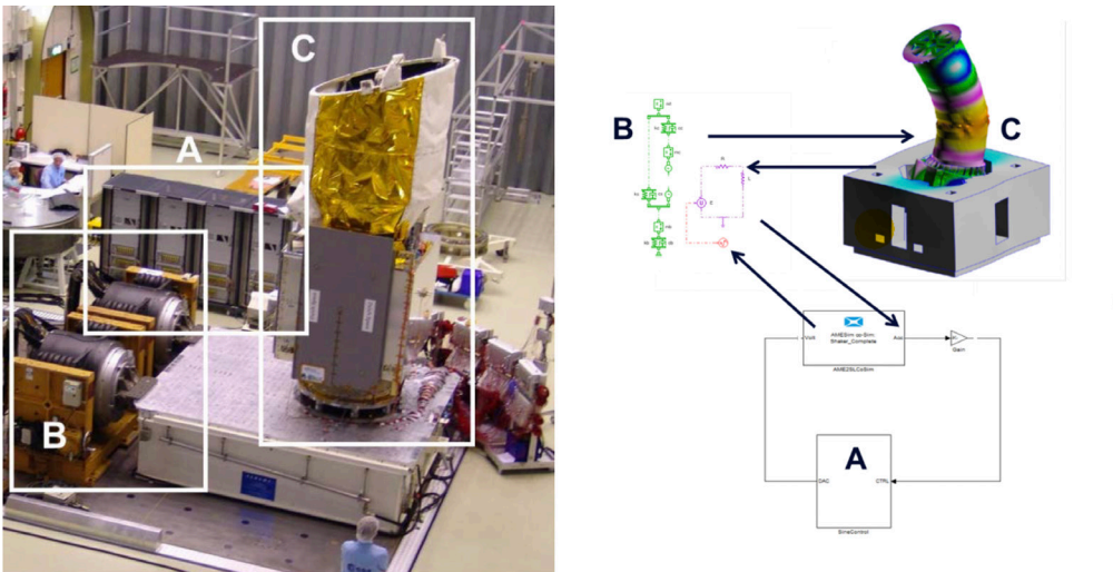
Figure 8. Vibration test facility (left) physical and (right) virtual representation. The different blocks are also marked: (A) Closed-loop vibration controller; (B) Vibration exciter(s); (C) Unit under test.
