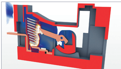
Example of Simcenter STAR-CCM+ multiphysics showing a cross-section of a low voltage circuit breaker simulation.
