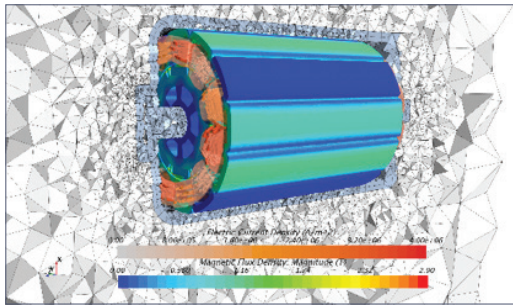
On the left is a realistic e-machine model in 3D. Mesh is 12.8 million elements. Right, performance on an Intel Xeon CPU E5-2698 version e3, 2.30 GHz, InfiniBand QDR.
