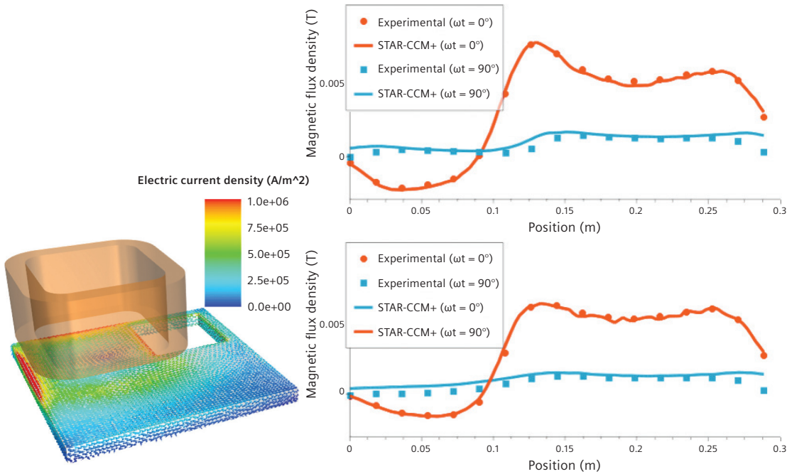
Results from Compumag society benchmark case showing electric current density analysis on the left and comparison with experimental results on the right.
