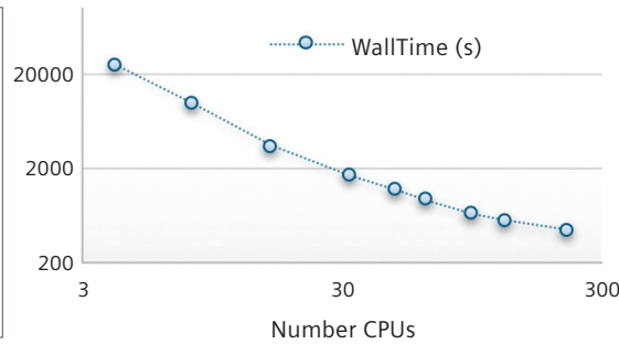
On the left is a realistic e-machine model in 3D. Mesh is 12.8 million elements. Right, performance on an Intel Xeon CPU E5-2698 version e3, 2.30 GHz, InfiniBand QDR.
