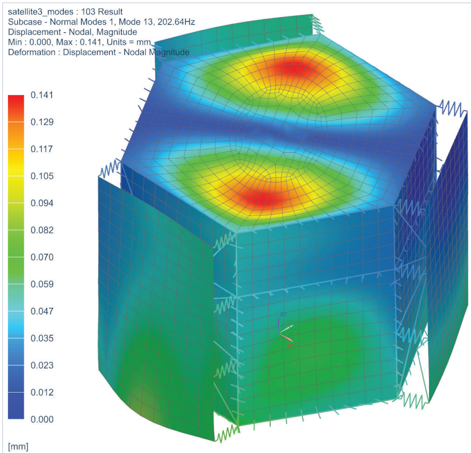
Figure 6. Dynamic behavior analysis of a satellite.
