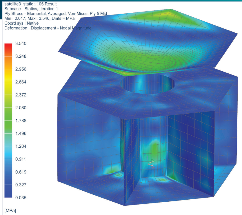
Figure 5. Simcenter 3D is used to run stress analysis to study failure behavior of composite materials.
