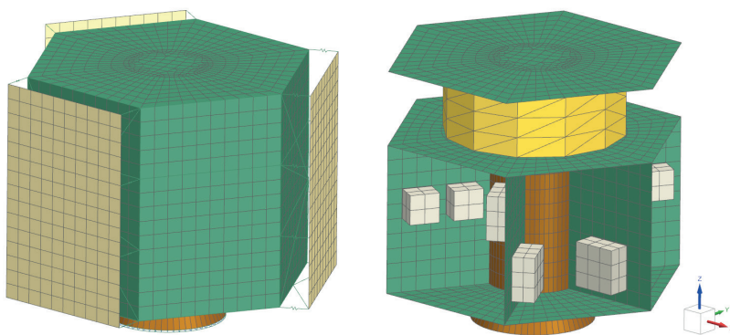
Figure 4. Visualization of a satellite and its equipment.
